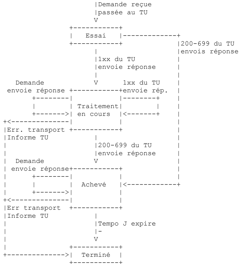
Figure 8 : Transaction serveur non-INVITE
