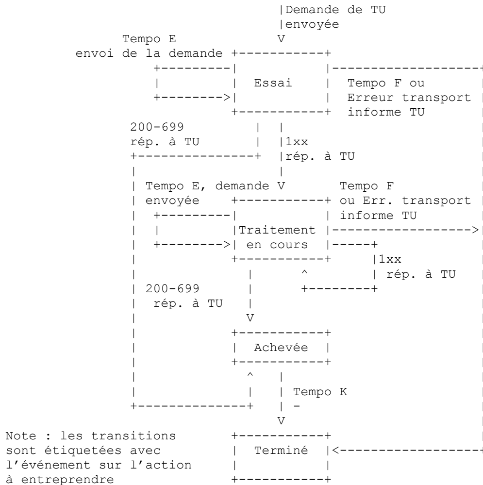
Figure 6 : Transaction client non-INVITE
