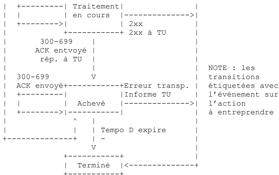
Figure 5 : Transaction client INVITE
