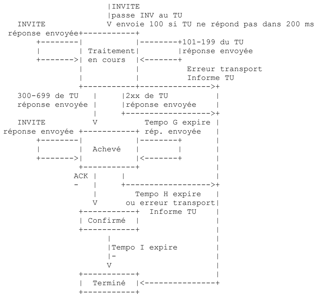
Figure 7 : Transaction serveur INVITE
