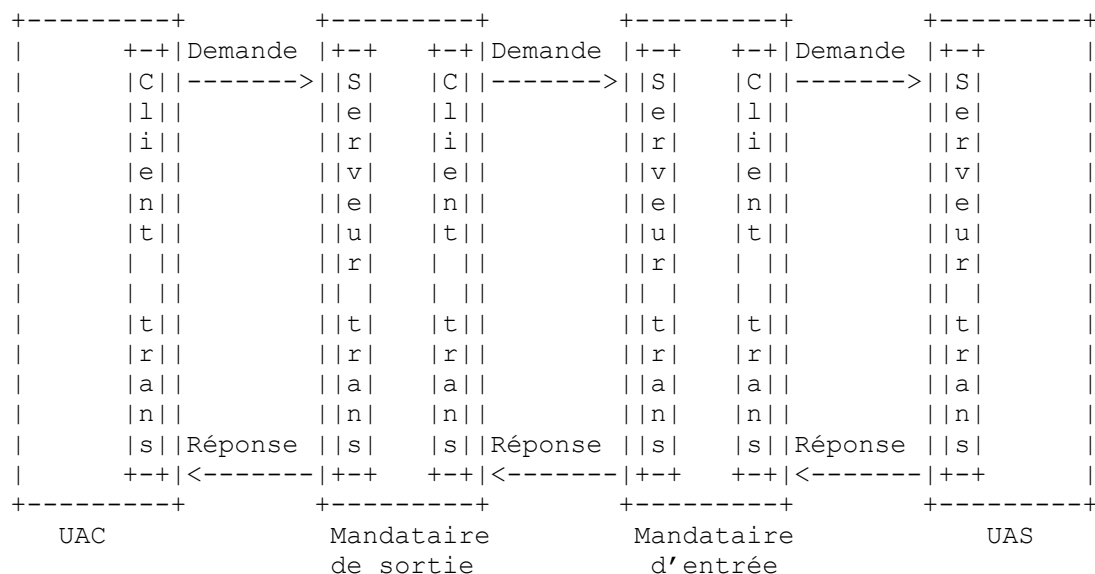
Figure 4 : Relations de transaction
