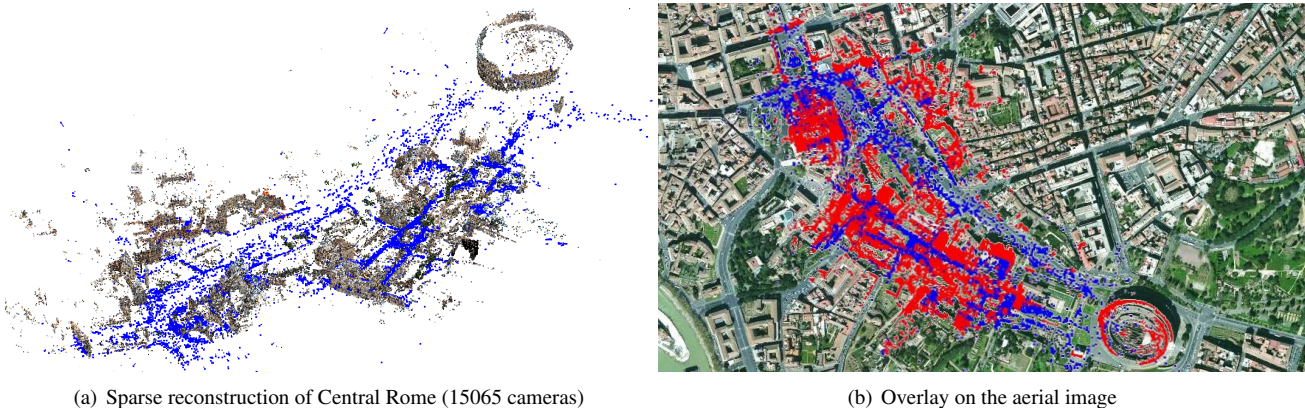
Figure 5. Our Rome reconstruction (the blue dots are the camera positions). The recovered structure is accurate compared to the map.
