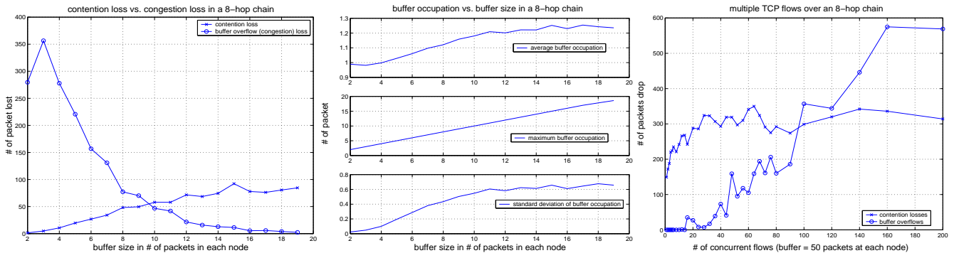
Figure 10: TCP loss transition Left: Buffer loss dominates when buffer is small; Contention loss dominates when buffer is large. Middle: Average and Maximum queue size of all nodes in the network. It shows that the average queue size occupancy at each node is very low. Right: Multiple concurrent TCP flows over an 8-hop chain. Buffer size at each node is set to 50 packets. The contention loss still dominates the packet losses.
