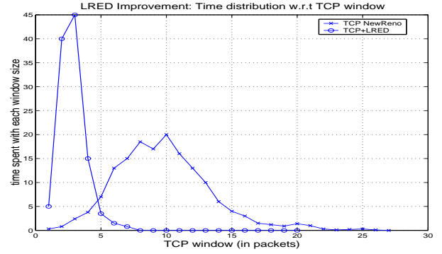
Figure 7: LRED stabilizes TCP window size around the optimal value. The Time distribution of instantaneous window size becomes narrower and sharper compared with TCP NewReno.
