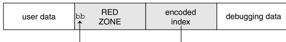
FIGURE 8-4 Redzone Byte at the Beginning of the Redzone
