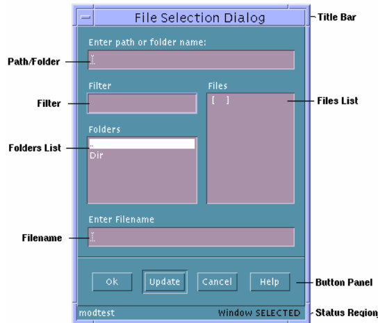
File Selection Dialog Object
