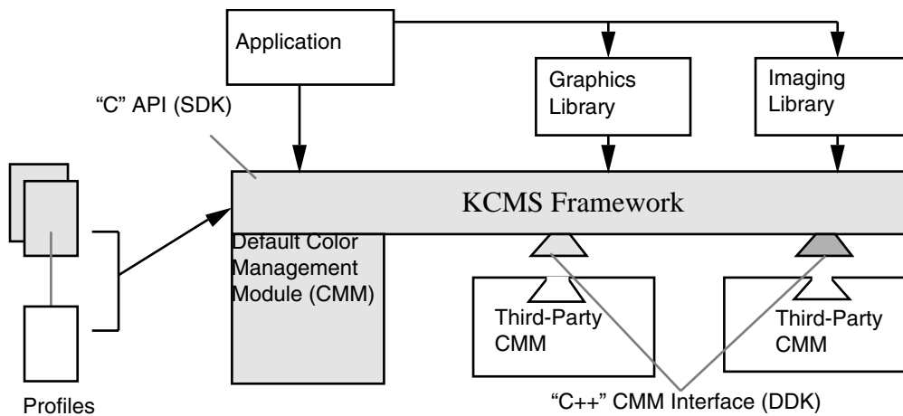
FIGURE 1-1 KCMS Architecture
