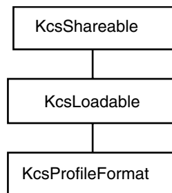
FIGURE 6-1 KcsProfileFormat Derivative
