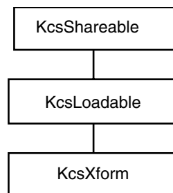
FIGURE 7-1 KcsXform Derivative
