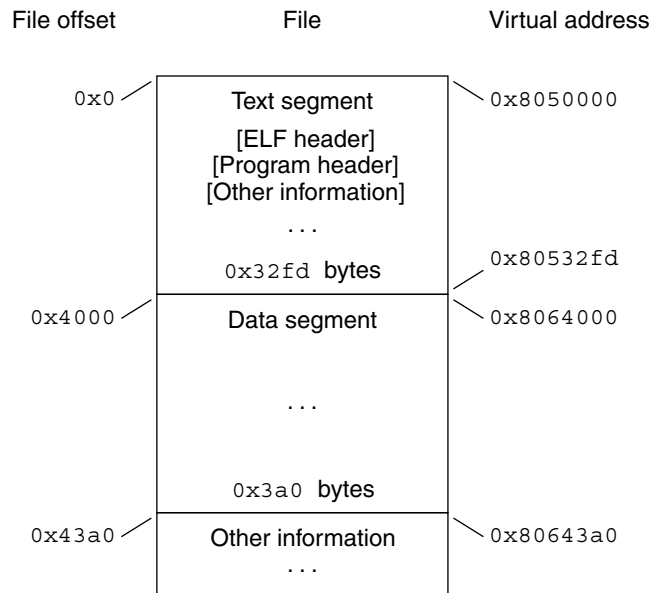
FIGURE 7-8 IA: Executable File (64K alignment)
