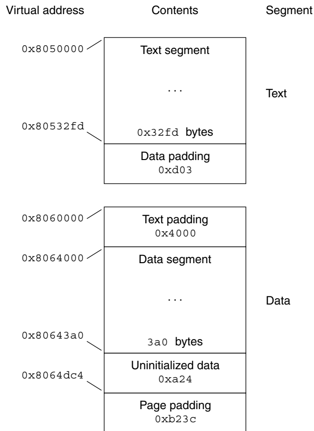
FIGURE 7-10 IA: Process Image Segments
