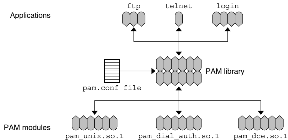
FIGURE 4-1 How PAM Works
