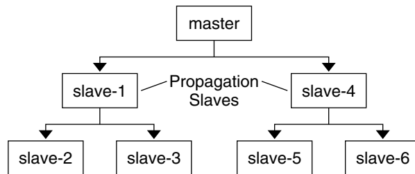
FIGURE 9-2 Example of Parallel Propagation Configuration
