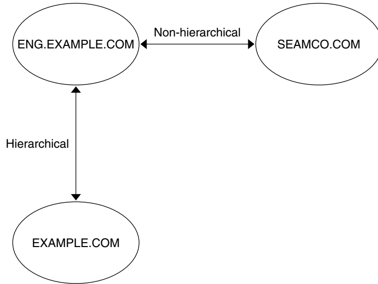
FIGURE 7-3 Realms
