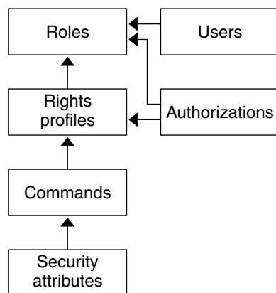
FIGURE 18-1 Solaris RBAC Element Relationships
