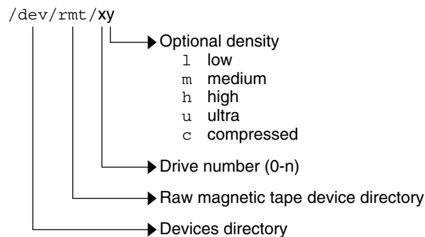
FIGURE 30-5 Logical Tape Device Names
