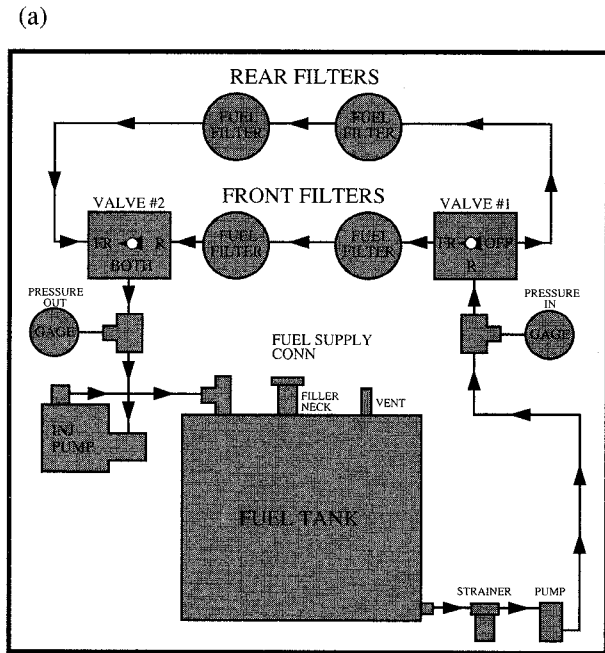
Figure 1. Editor scene (a), and four frames from its graphical history (b).
