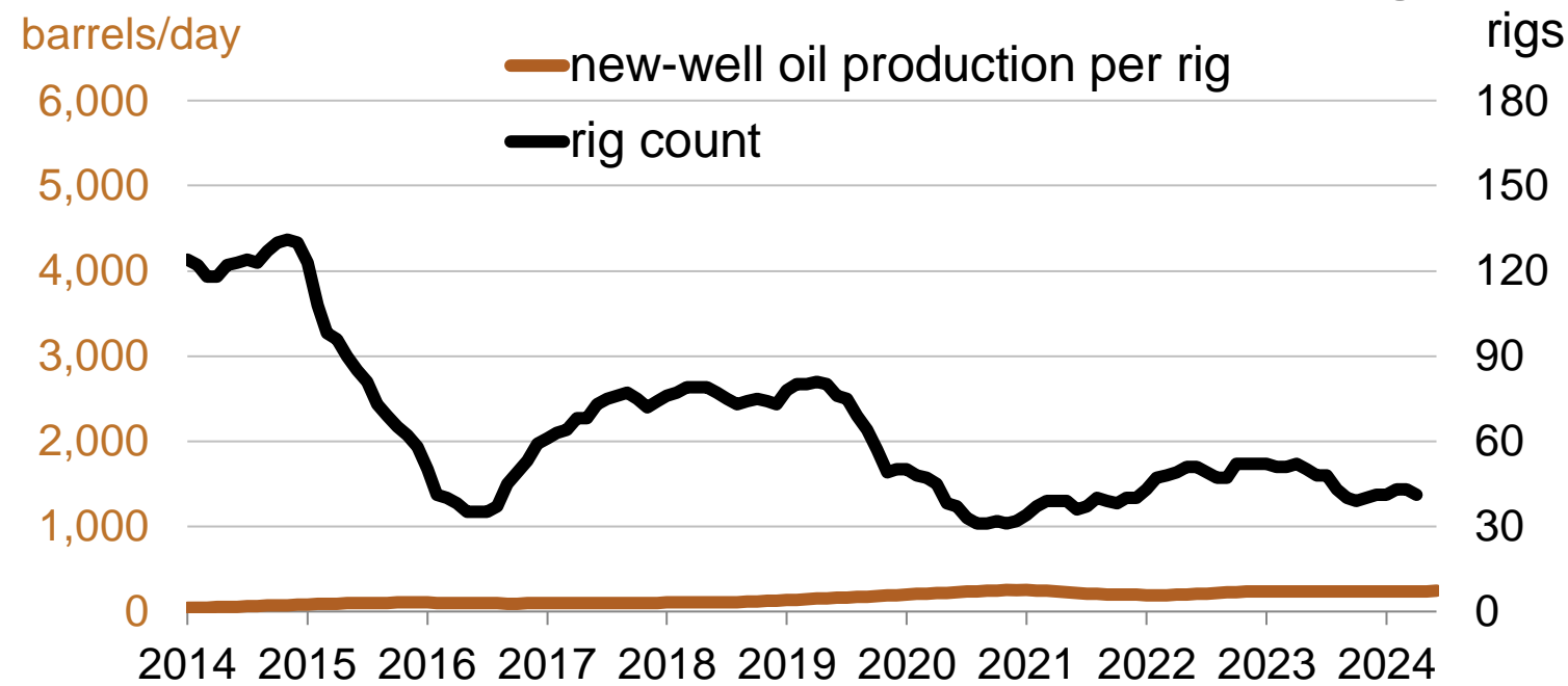
Appalachia Region New-well oil production per rig
